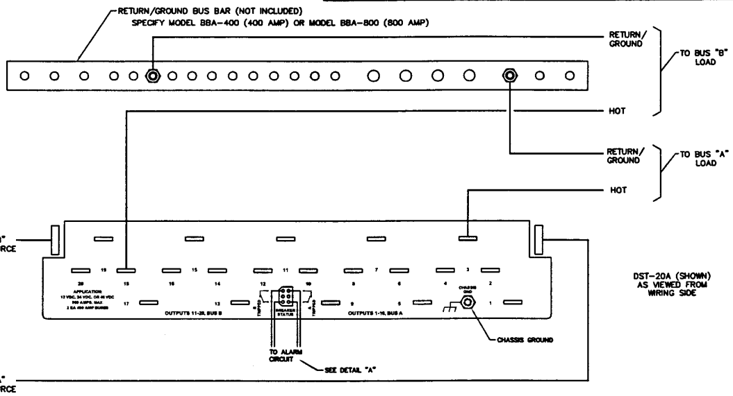
-SPLIT BUS INSTALLATION, MODEL DST-20A ONLY-
