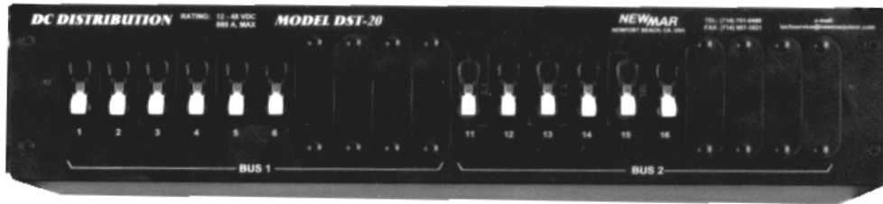
Model DST-20A pictured with 12 optional breakers installed
