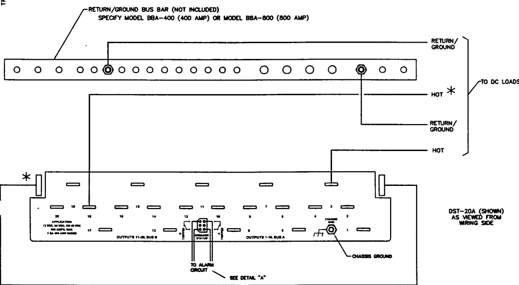
-SINGLE BUS INSTALLATION-
